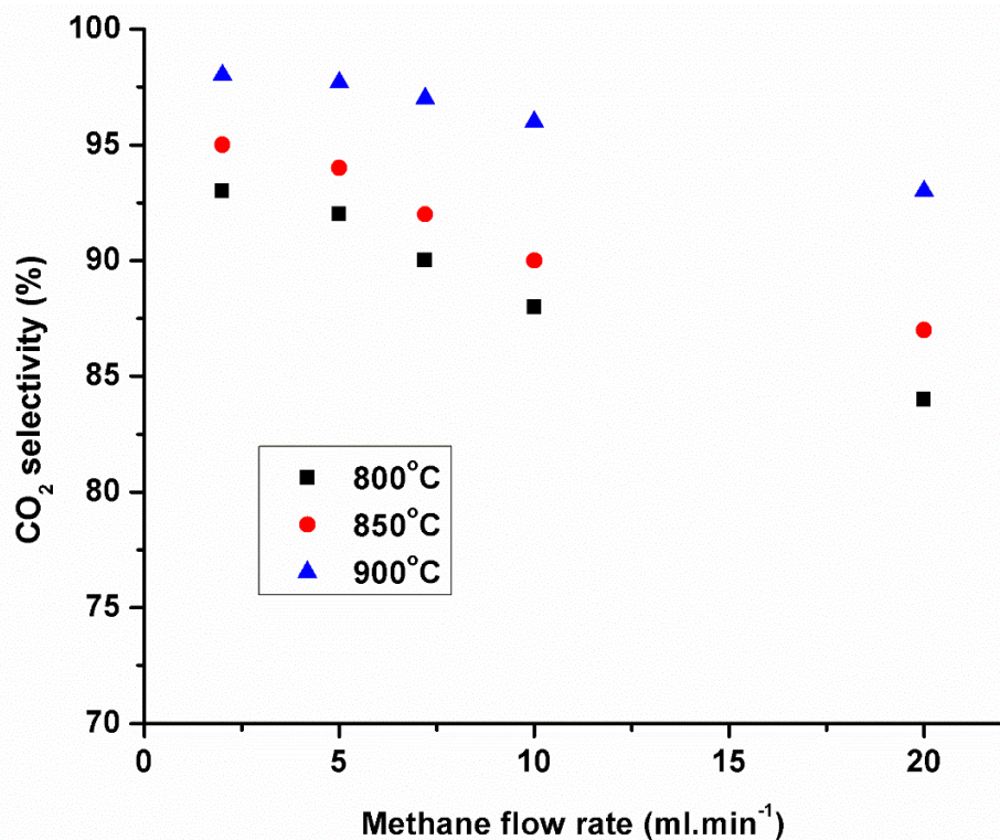
Figure 4.5 CO 2 selectivity of SSC planar OTM with an additional porous catalyst layer subjected to methane flow rates ranging from 2 to 20 mL·min -1 while held at membrane temperatures ranging from 800 to 900°C
