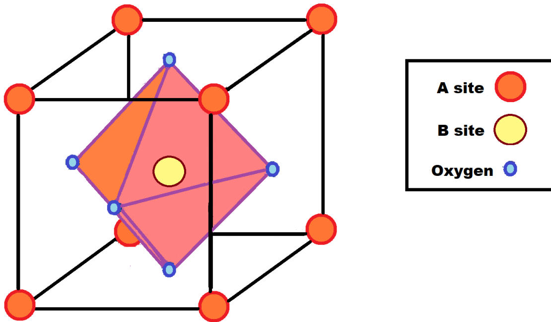
Figure 1.4 Ideal perovskite structure
